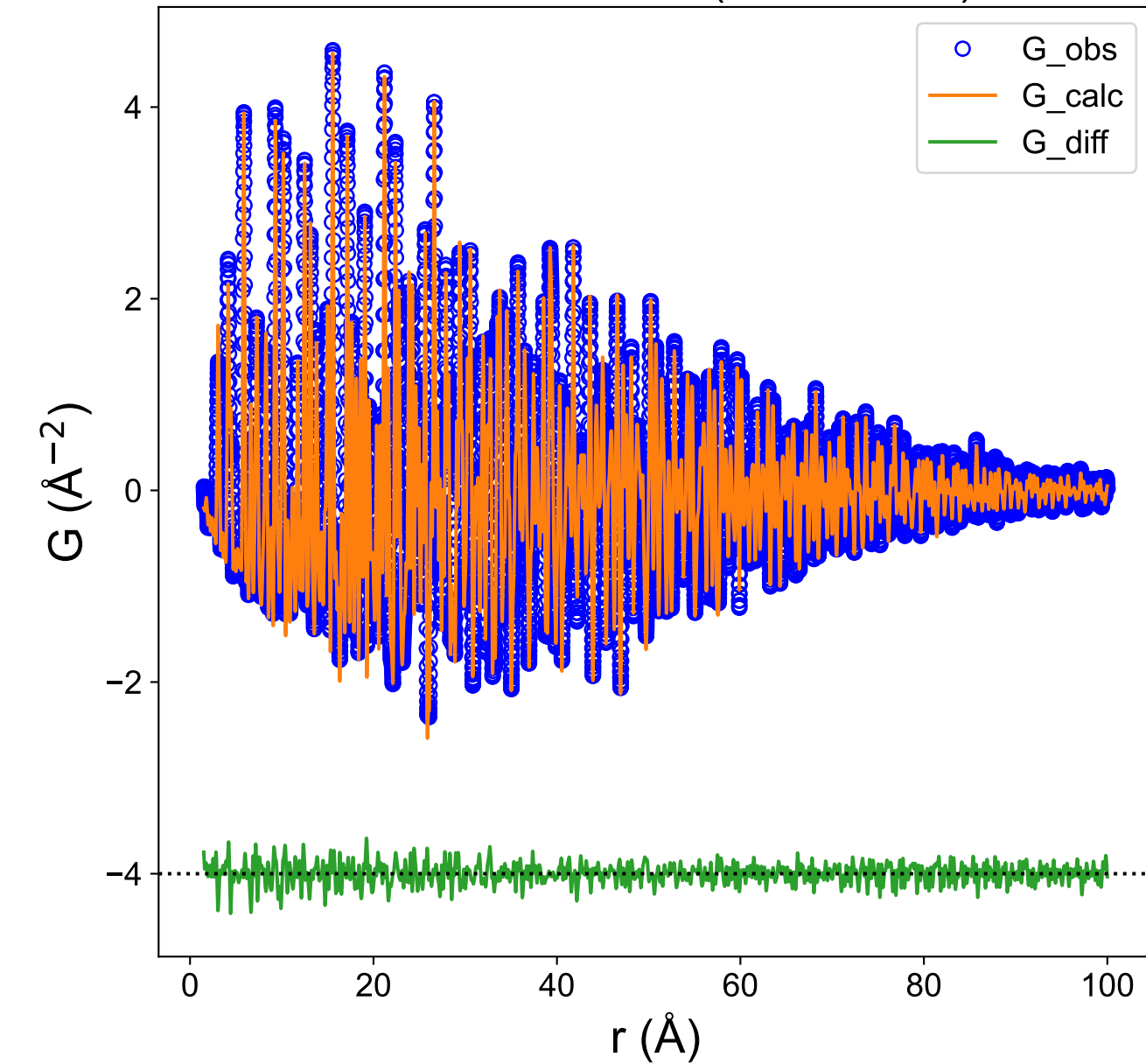
PDF Data and Fit (Rw = 0.112)
